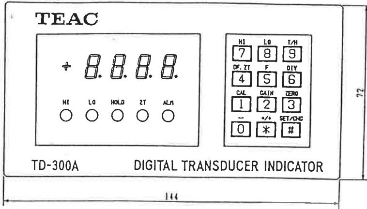
FRONT PANEL
