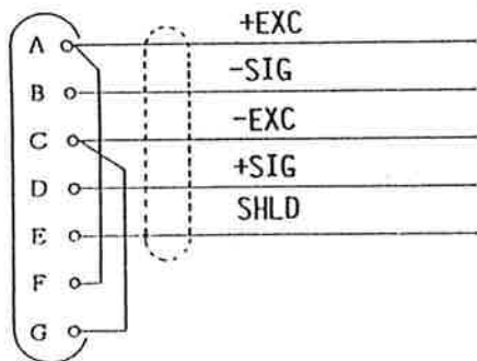
4 CORE CABLE
