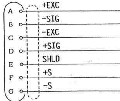
6 CORE CABLE
