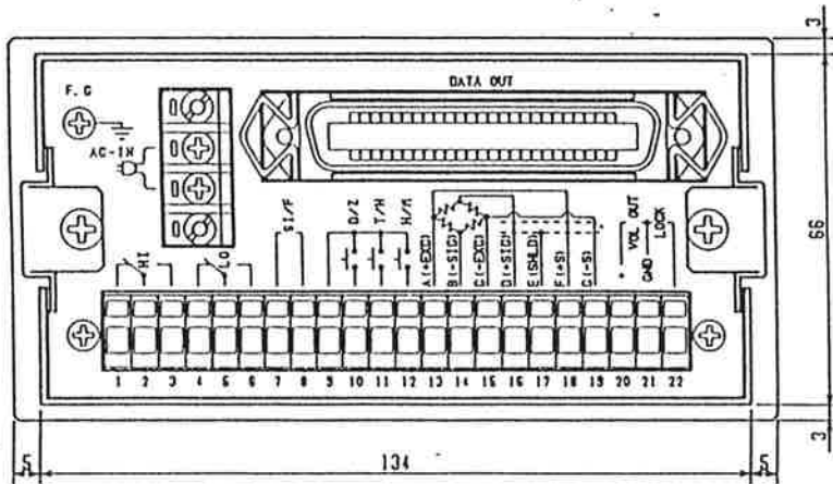
REAR PANEL
